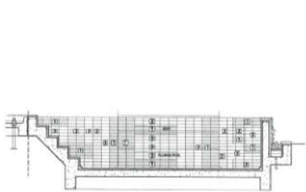
CERAMIC TILE PATTERN SECTION A SCALE 1:25 (A4:10)
