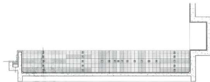
CERAMIC TILE PATTERN SECTION C SCALE 1:25 (A4:10)
