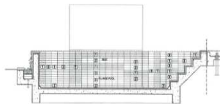
CERAMIC TILE PATTERN SECTION B SCALE 1:25 (A4:10)
