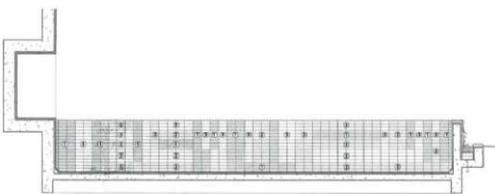
CERAMIC TILE PATTERN SECTION D SCALE 1:25 (A4:10)
