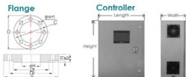
HG-20592 PN 1.0 Mpa Standard flange size
