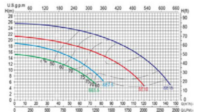
Remark: The performance curve above is for 50Hz models.
